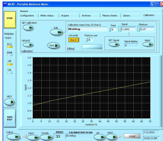
Calibration task in AK30 program
